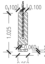
2 TYP. SILL DETAIL SCALE NTS
