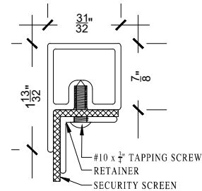
1 TYP. HEAD DETAIL SCALE NTS
