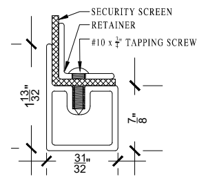
2 TYP. SILL DETAIL SCALE NTS
